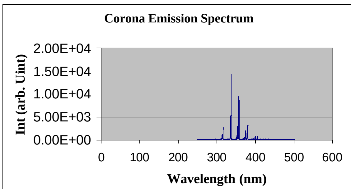
Figure 2: Corona emission spectrum from a point-plane configuration
